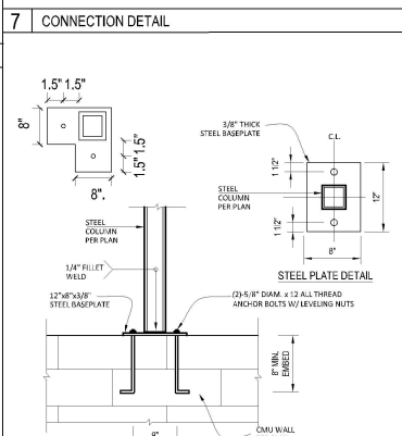
6 CONNECTION DETAIL
