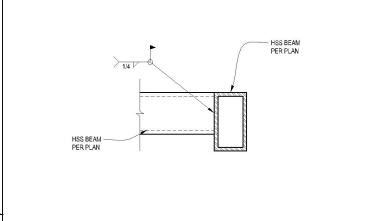
8 CONNECTION DETAIL
