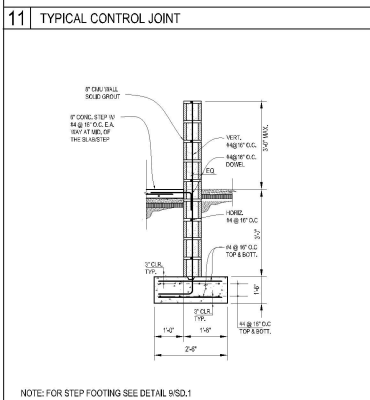
11 TYPICAL CONTROL JOINT
