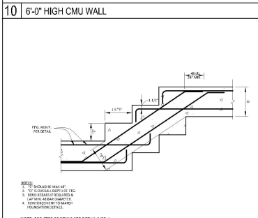
9 STEPPED FOOTING BELOW GRADE
