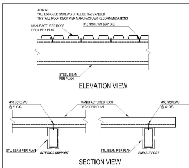
12 CONNECTION DETAIL
